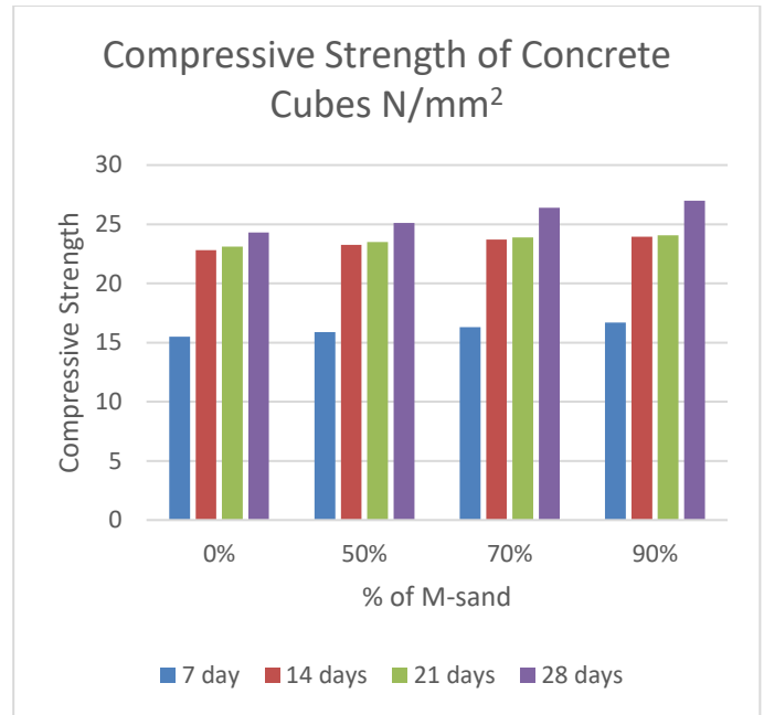
Fig 4 : Compressive Strength
