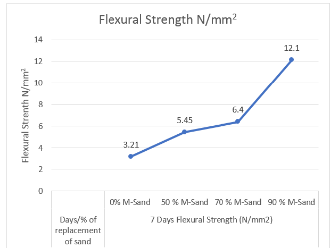
Fig 5 : Flexural Strength
