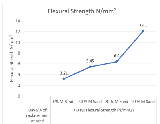
Fig 3 : Flexural Strength
