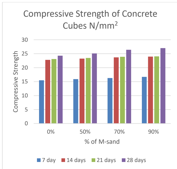
Fig 2 : Compressive Strength
