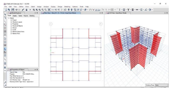
Case II Shear walls at the Corners
