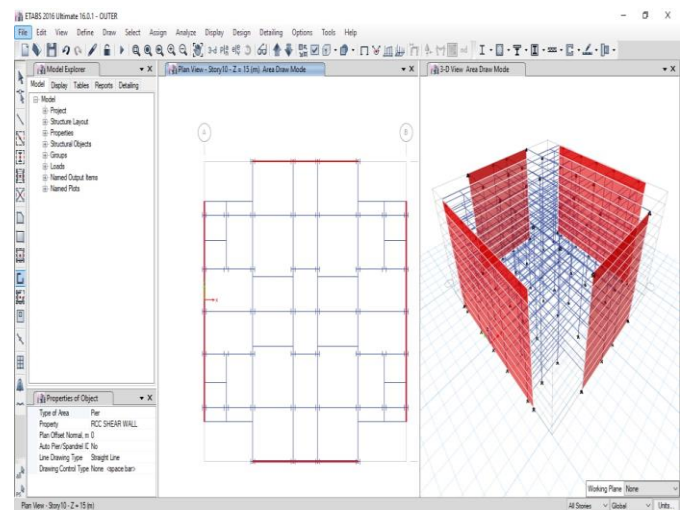
Case II Shear walls at the Corners
