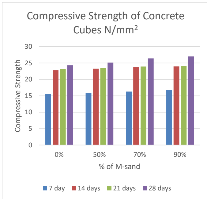
Fig 2 : Compressive Strength
