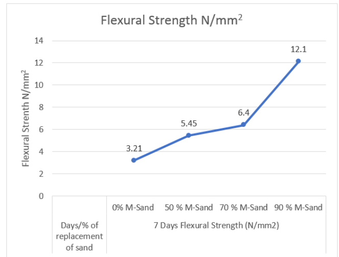
Fig 3 : Flexural Strength
