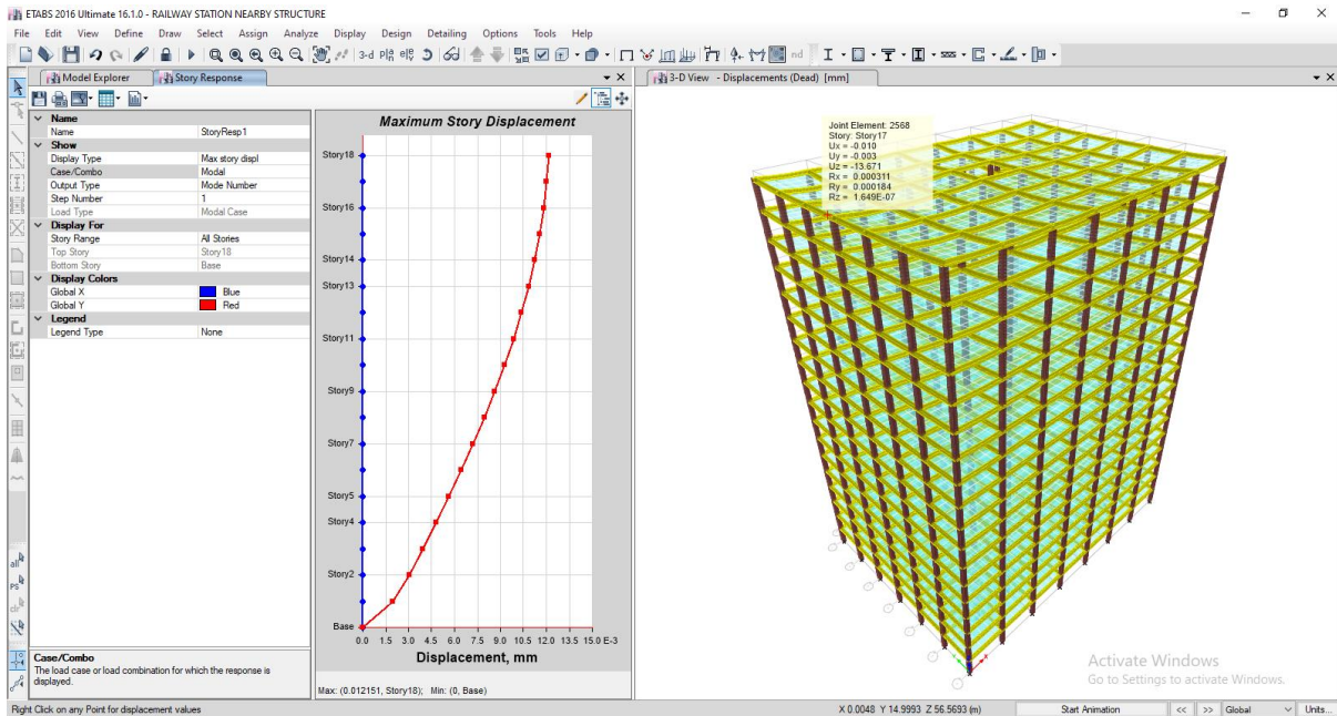
Fig 13 Stress Analysis
