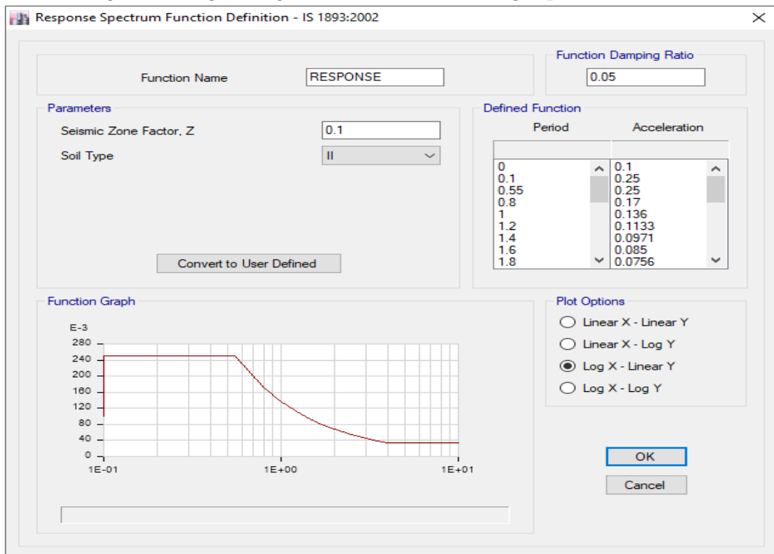
Fig 11 Response Spectrum Function
