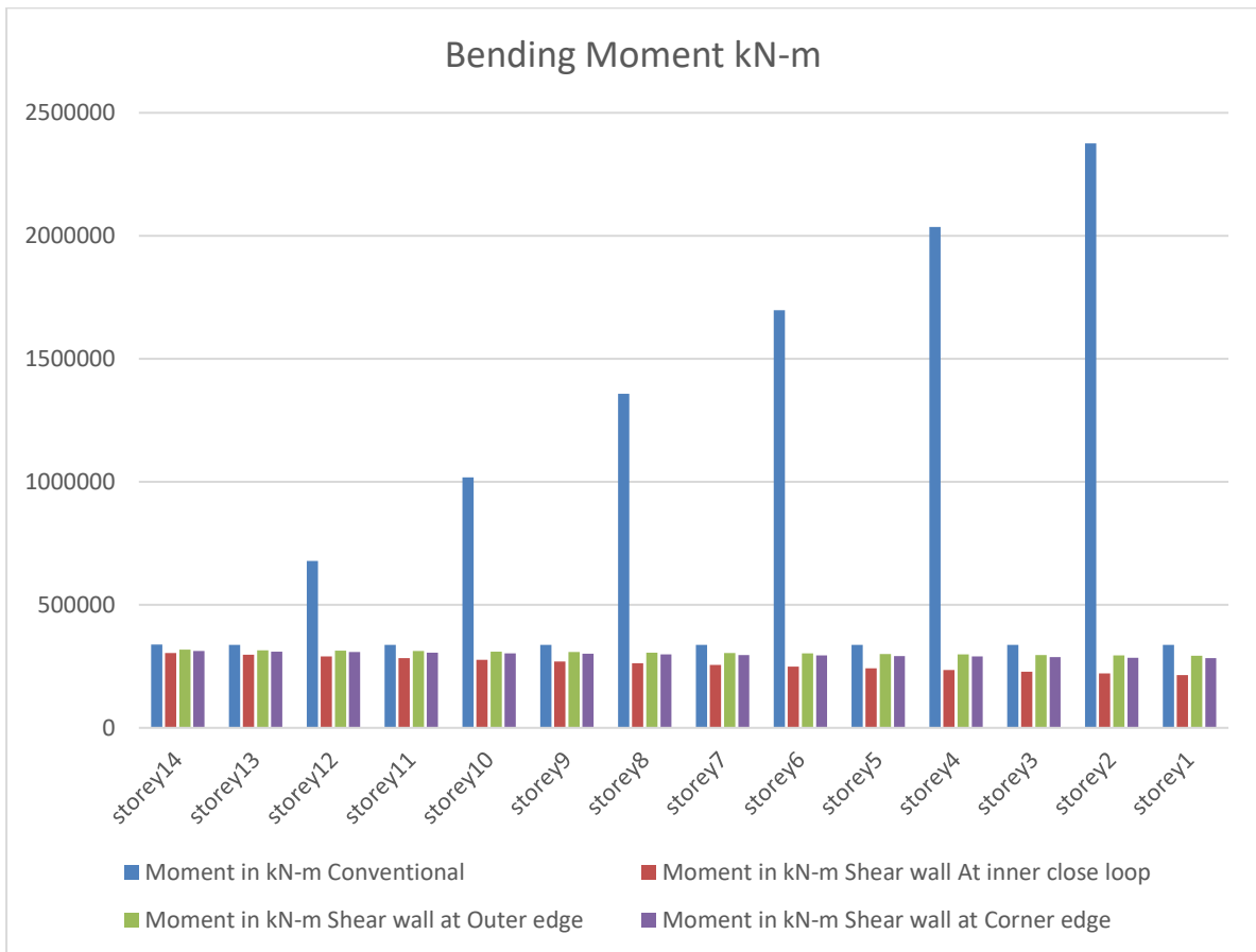
Fig 6: Moment
