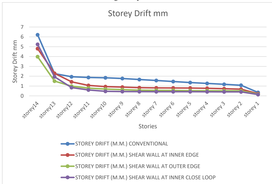
Fig 3: Drift
