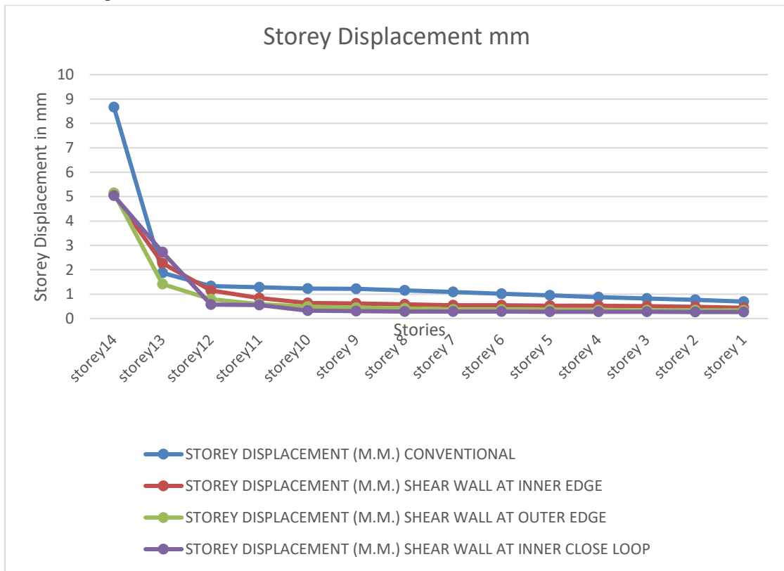
Fig 2: Displacement
