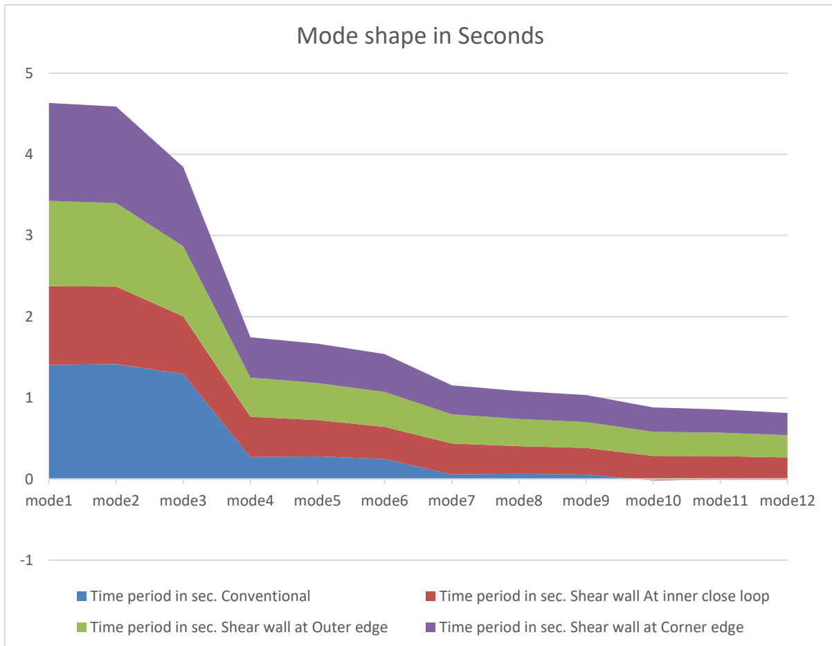
Fig 5: Mode Shape
