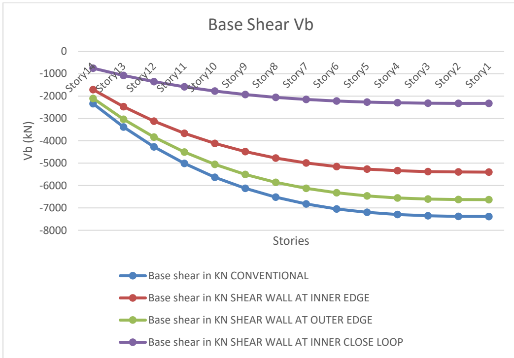
Fig 4: Base Shear
