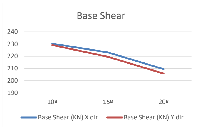
Fig 11 Base Shear
