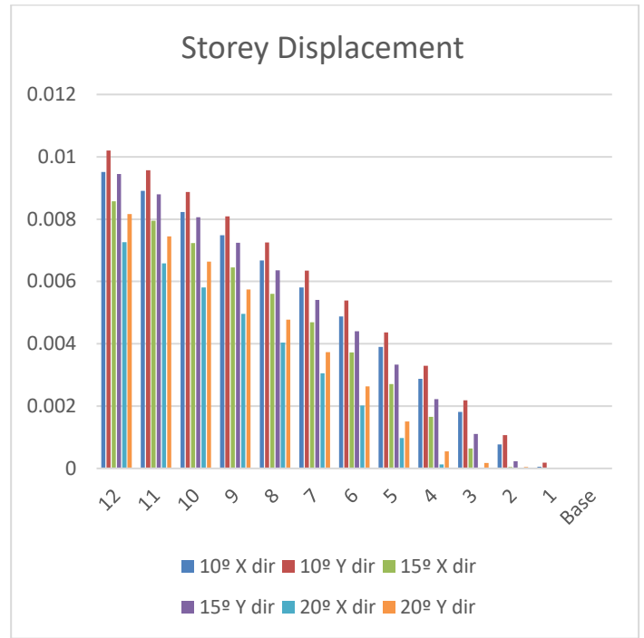
Fig 12 Storey Displacement
