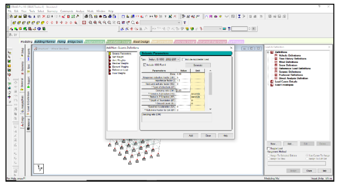
Fig 8 Assigning seismic load as per IS 1893- 2002
