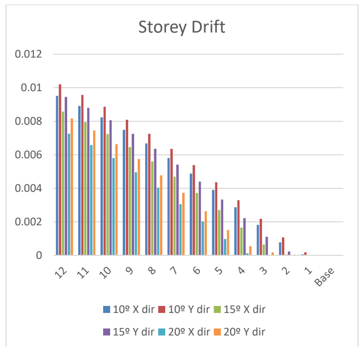
Fig 13 Storey Drift
