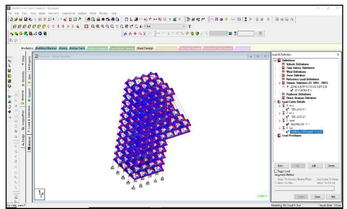
Fig 6 Assigning Support steel cables to the extension
