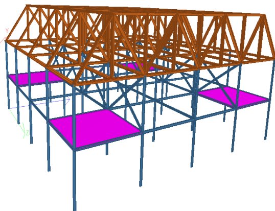
Figure b) Structure with Dampers and Bracings
