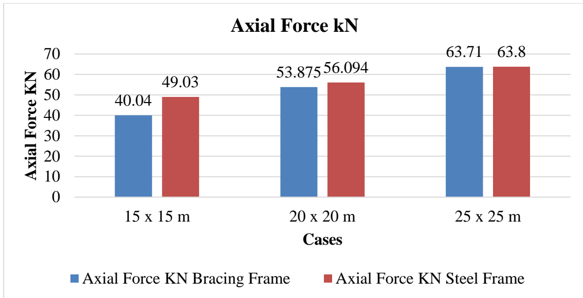
Fig 10: Axial Force
