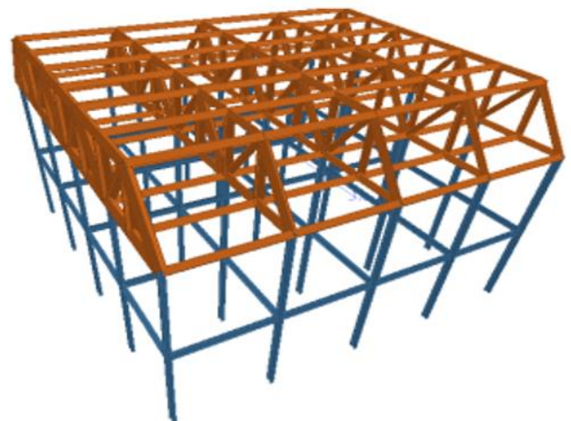
Figure a) General Structure
