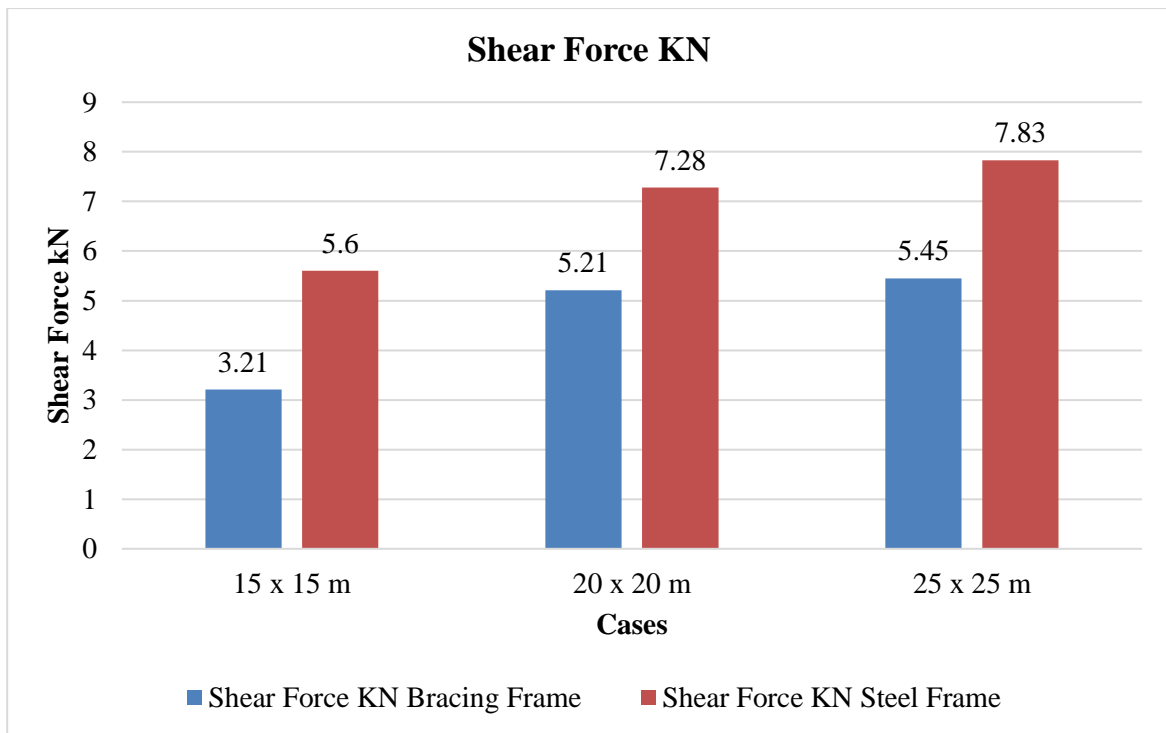
Fig 11: Shear Force
