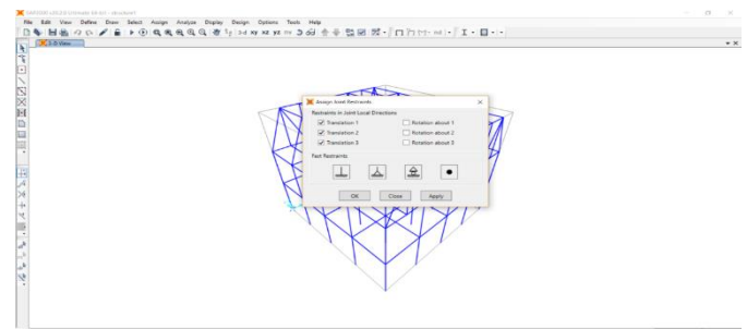
Figure 5. Assigning support conditions
