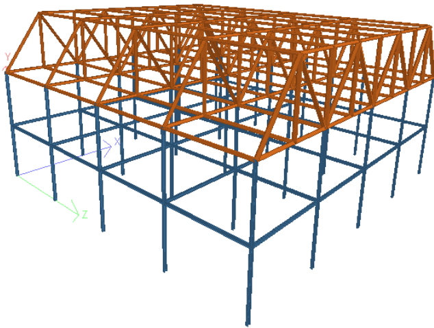
Figure a) General Structure
