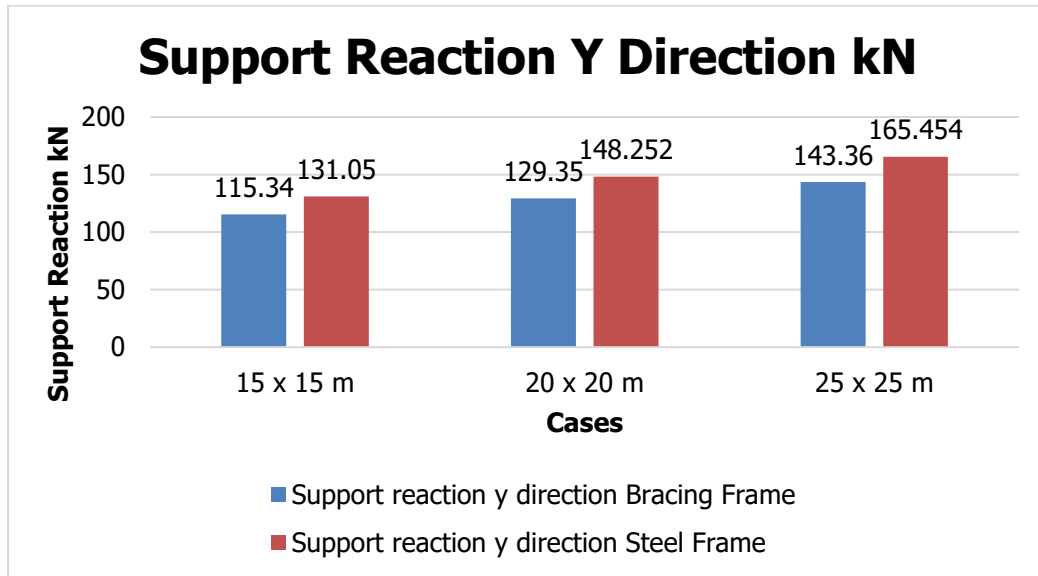
Fig 8 : Support reaction
