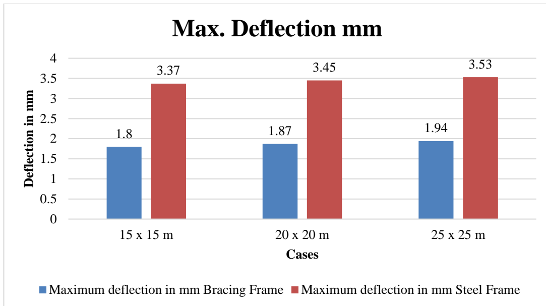
Fig 9 : Deflection
