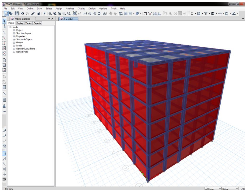
Fig 7: Hybrid structure
