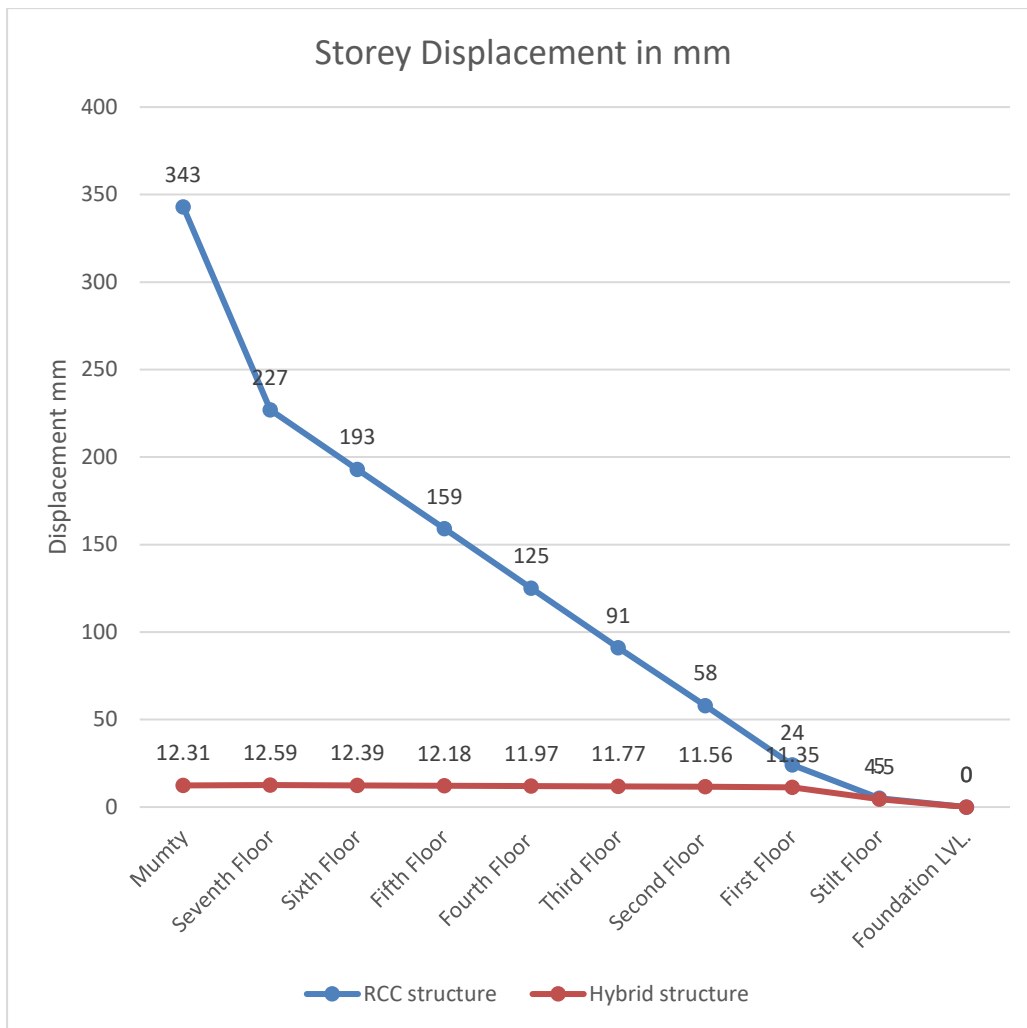
Fig 8: Storey Displacement
