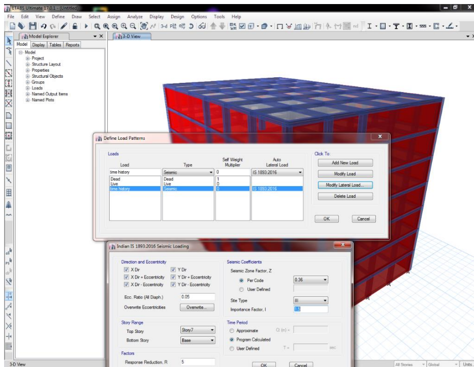
Fig 5: Load Condition
