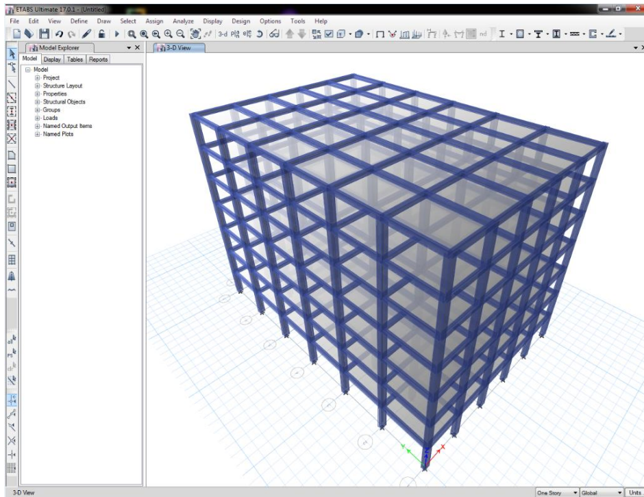
Fig 6: Bare Frame
