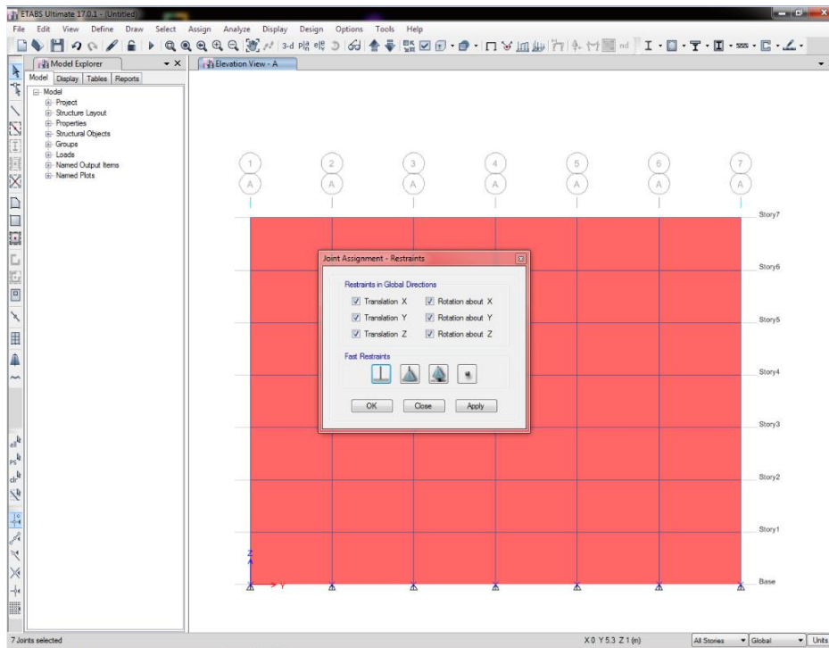
Fig 3: Assigning fixed end condition
