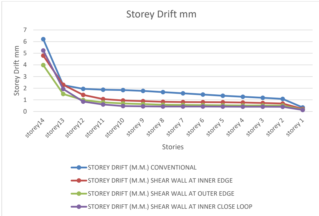
Fig 3: Drift
