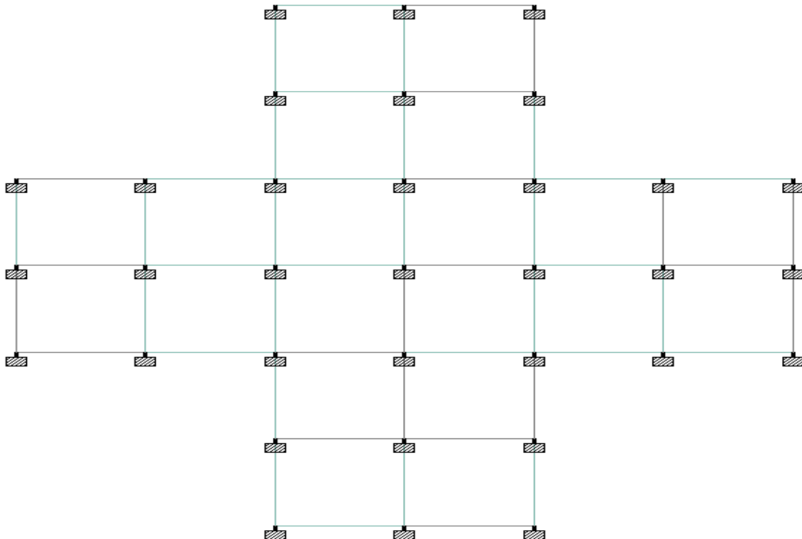
Fig 1: Plan of plus shaped structure
