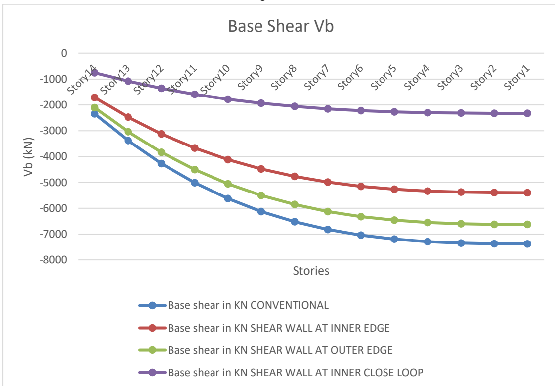
Fig 4:Base Shear
