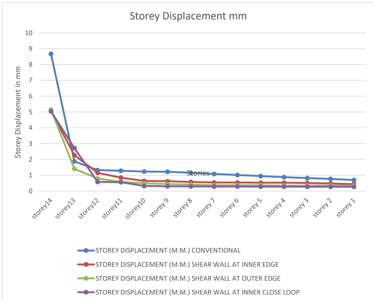
Fig 2: Displacement
