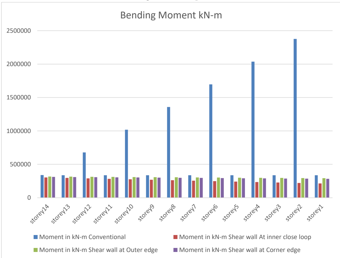
Fig 6: Moment
