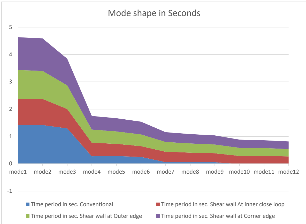
Fig 5: Mode Shape
