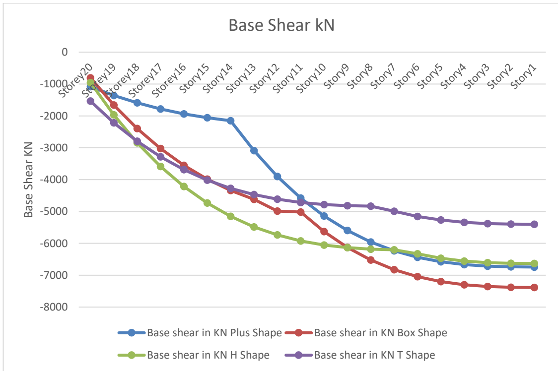
Fig 7: Base Shear
