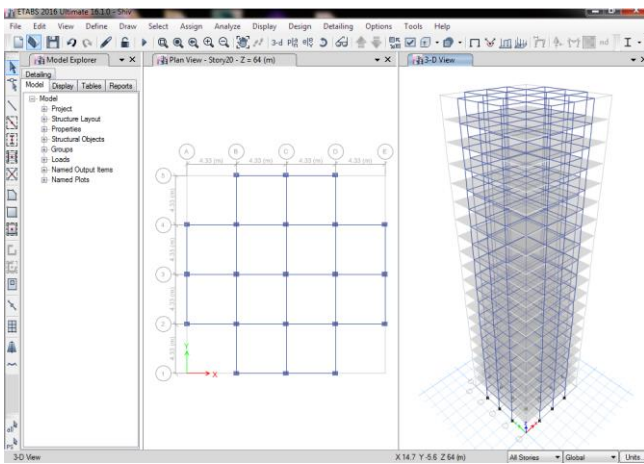
Fig 3 : Plus Shape Structure
