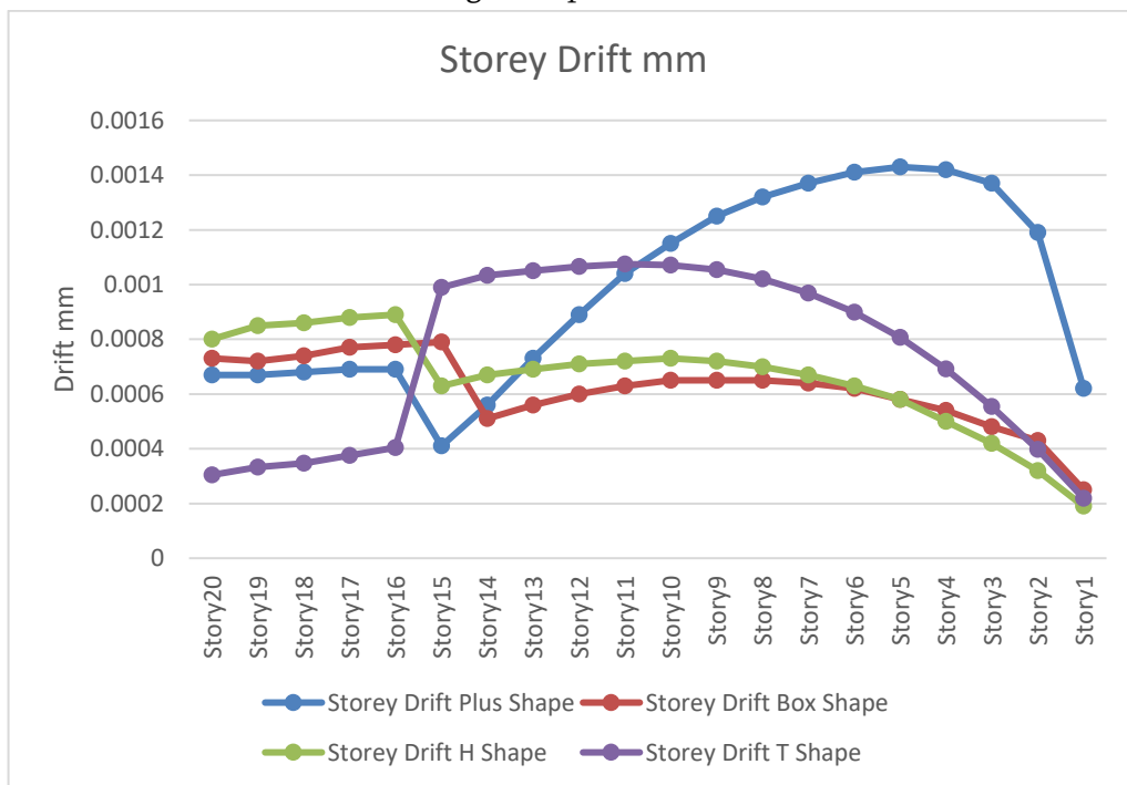
Fig 6: Drift
