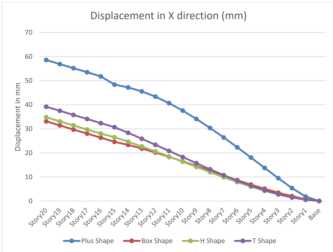
Fig 5: Displacement
