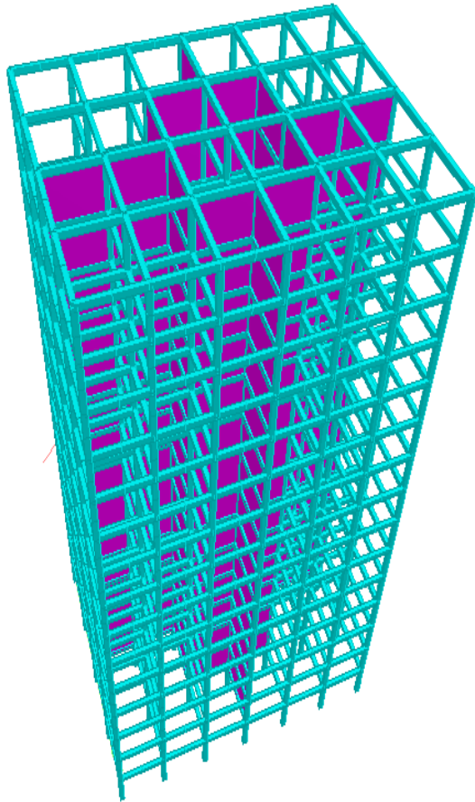
Figure 3. Modelling of Outrigger
