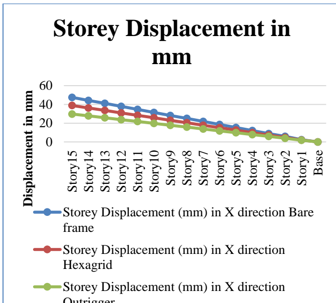
Fig 10 : Storey Displacement in mm
