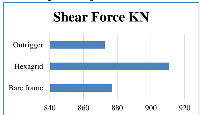
Fig 8 : Shear Force in KN
