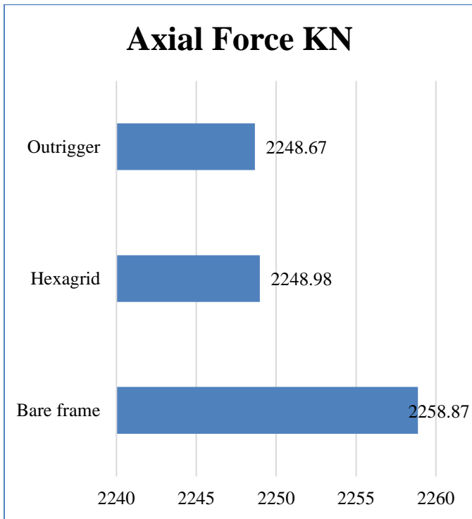
Fig 9 : Axial Force in KN
