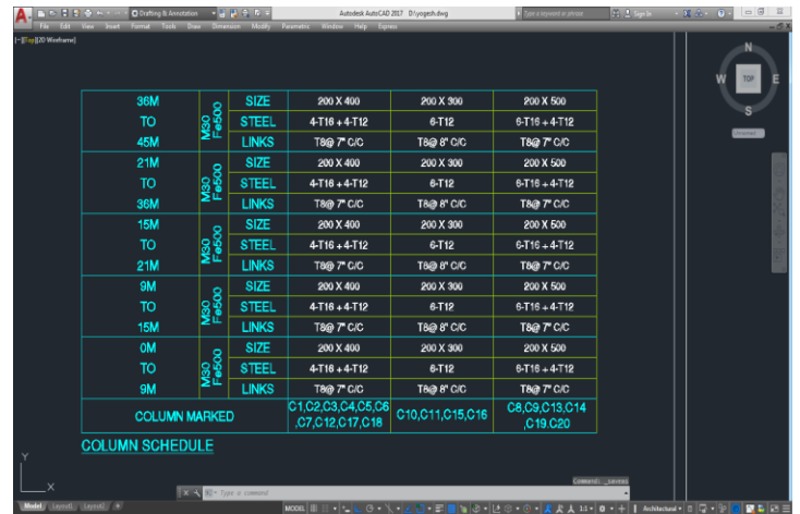
Fig 11 : Detailing of structure in autocad
