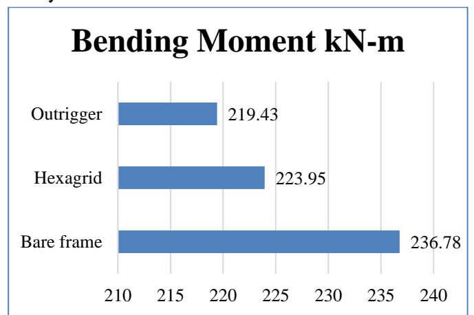
Fig 7 : Bending moment in KN-m
