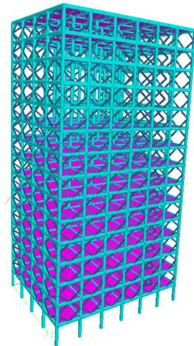
Figure 2. Modelling of Hexa-Grid
