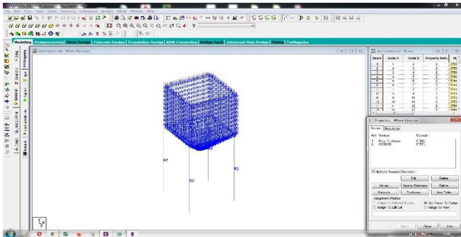
Fig 3 Assigning Steel Properties as per IS 2062 (2011)
