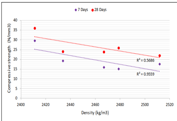
Fig 6: Regression graph between Compressive strength & 1 Day-density.
