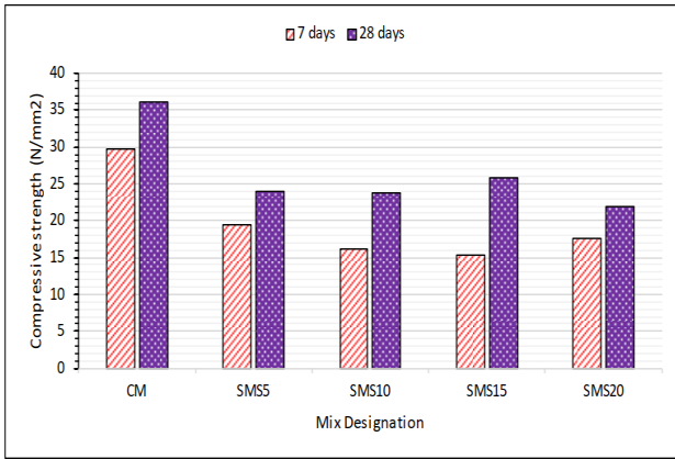
Fig 5: Compressive strength in 7 & 28 Days.
