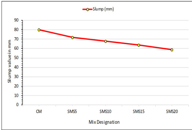
Fig 3: Slump cone graph of Mix design.
