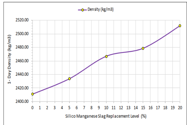
Fig 4: 1 Day-density graph of concrete cubes.
