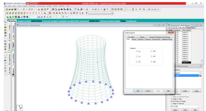
Fig 4 : Assigning Support condition
