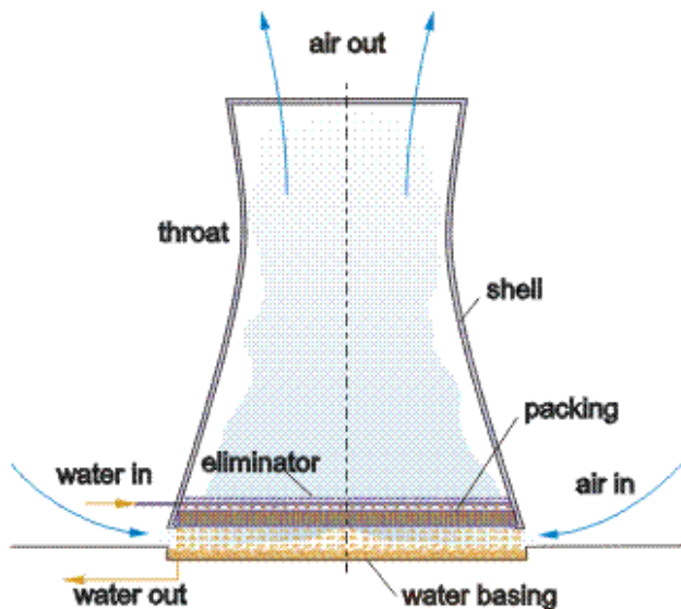
Fig 1: Cooling Tower
