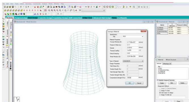
Fig 3 : Assigning material and section properties
