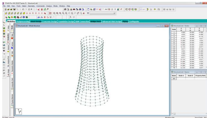
Fig 2 : Modelling of Cooling Tower using Staad.Pro.
