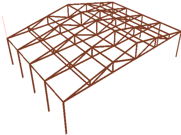
Fig 5 : Modelling of the structure in staad.pro
