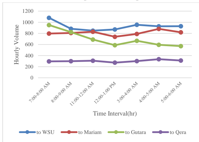
Figure-2: Traffic volume for Existing Bus station in Friday
