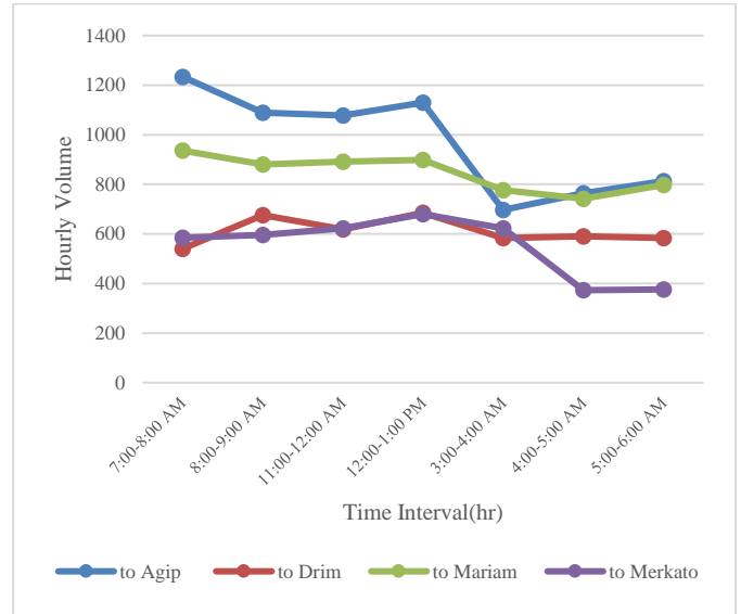
Figure-3: Traffic volume for 21-Mazoria in Monday
