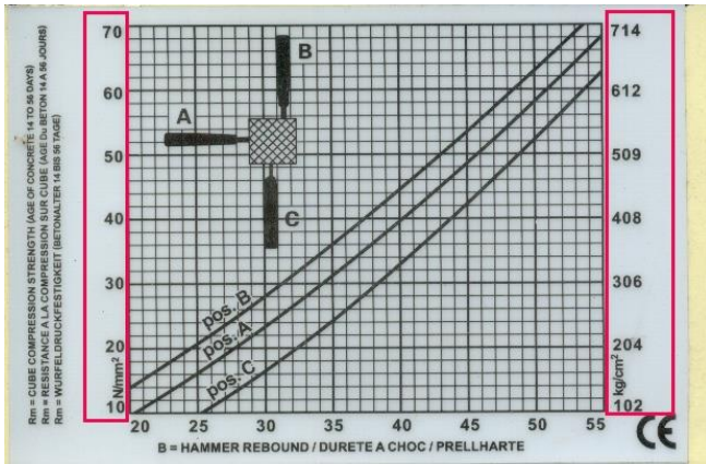
Fig:1 NDT Graph
