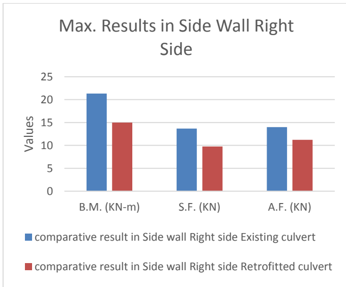
Fig 10 Right hand side wall
