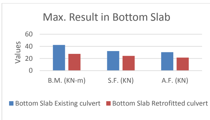
Fig 12 Comparative results on Bottom slab
