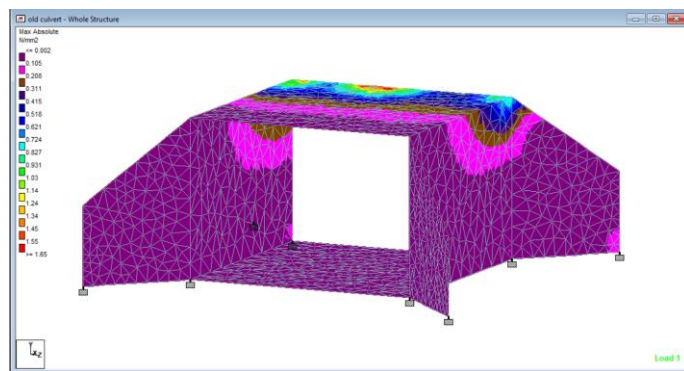
Fig : 2 stress distribution
