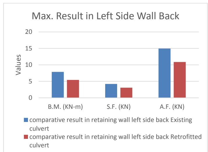
Fig.4 Retaining wall Left side
