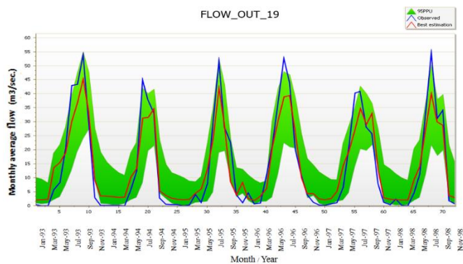
Figure 4 : The result of calibration for average monthly stream flows.
