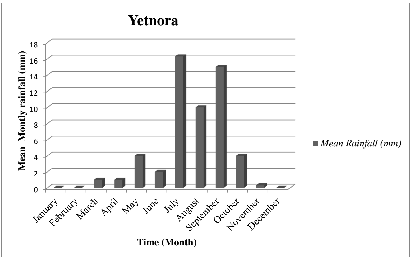
Figure 2 : Mean monthly rainfall distribution of selected meteorological stations in and around the watershed.
