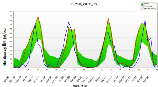
Figure 5 : The result of Validation for average monthly stream flows.
