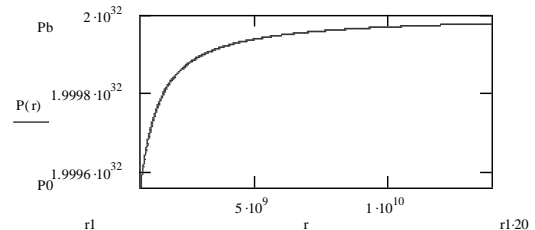
Fig. 2. Radial distribution of pressure of air for the Sun.
