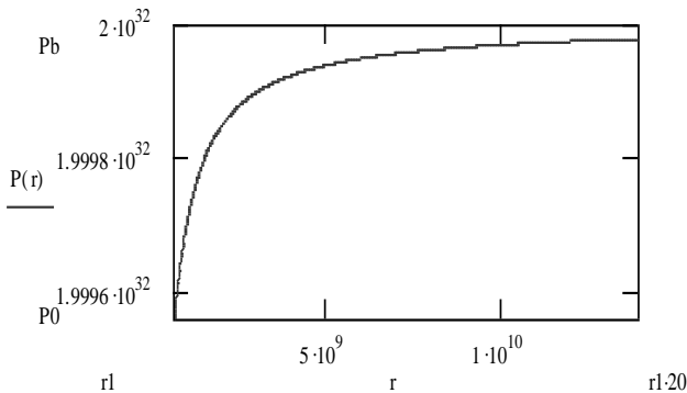
Fig.2. Radial distribution of ether pressure for the Sun.
